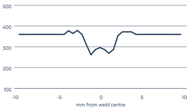
Figure 1. Example of hardness profile across a transverse weld in a IPCO 1400SAF belt.
